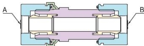
PANEL MOUNT REDUCING UNION CONNECTOR
